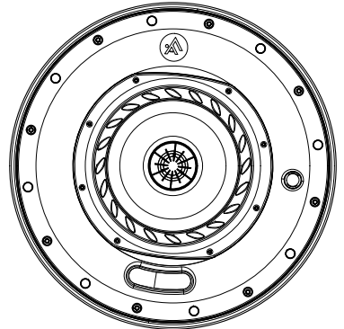
Bottom View (with grille removed)
