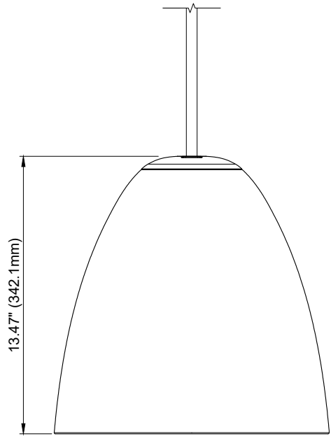
Side View (with hanging cable)
