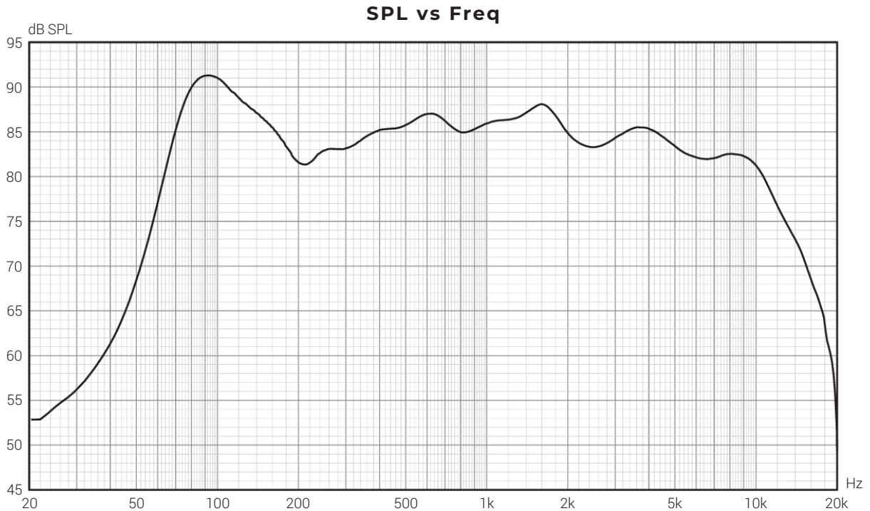
LookHear Frequency Response with 2.83V at a 4m (13.1 ft) distance and at a listening position of 1.7m (5.5 ft) high with DSP applied.
